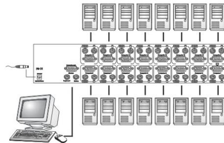
Up to 128 computers/servers can be controlled via one set of keyboard, video display, and mouse through a cascaded Minuteman KVM
